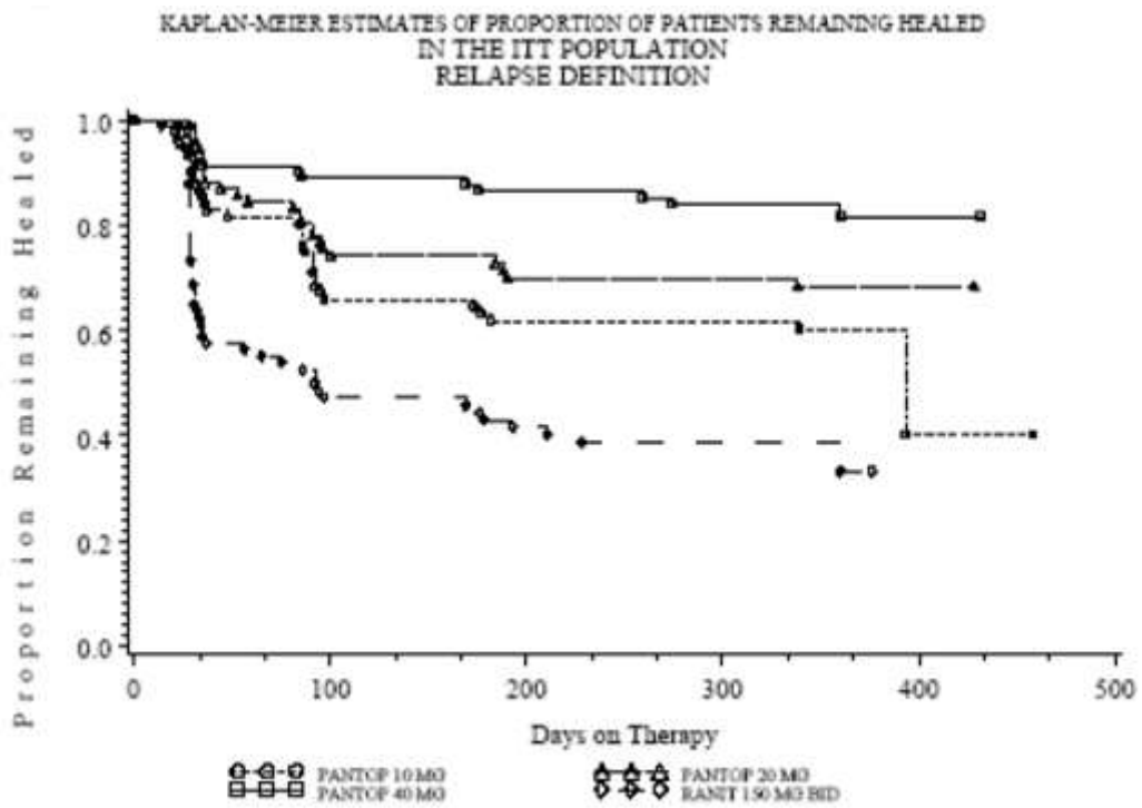
Kaplan-Meier plot; 3001A1-303-US
