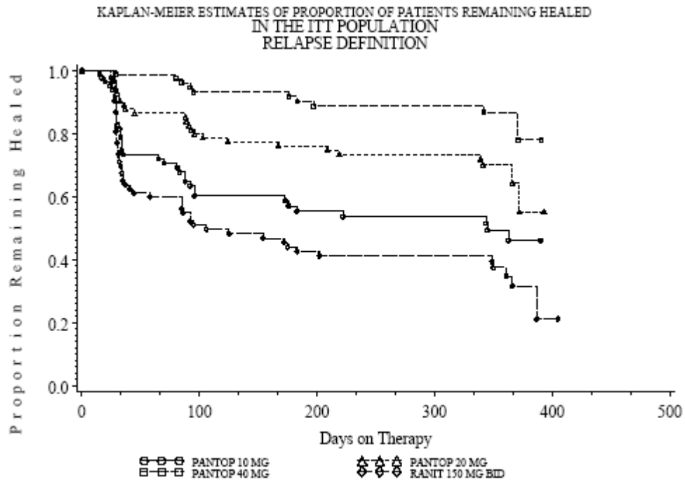
Kaplan-Meier plot; 3001A1-302-US
